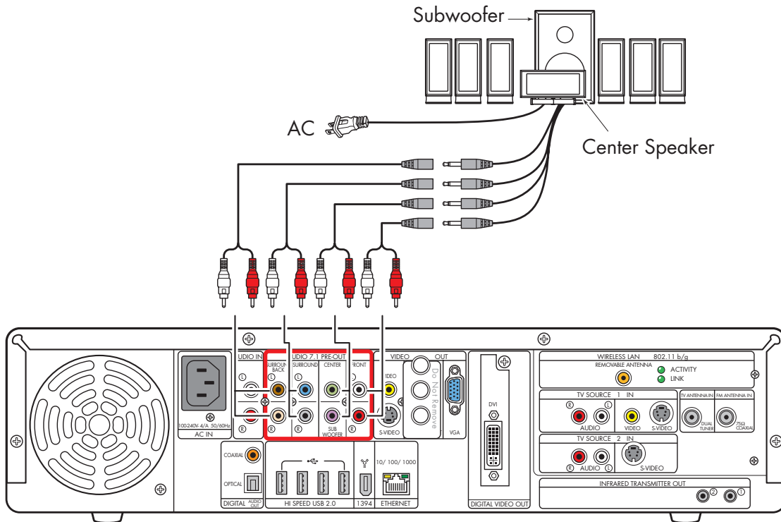
Typical 7.1 powered speaker installation
